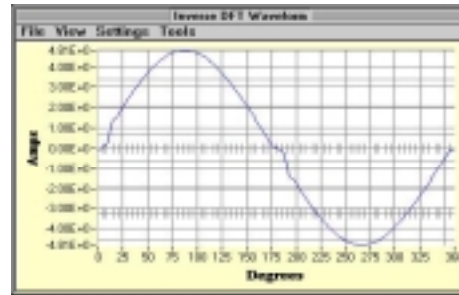
Input AC Current Waveform (I THD = 3% at 100% Load)
